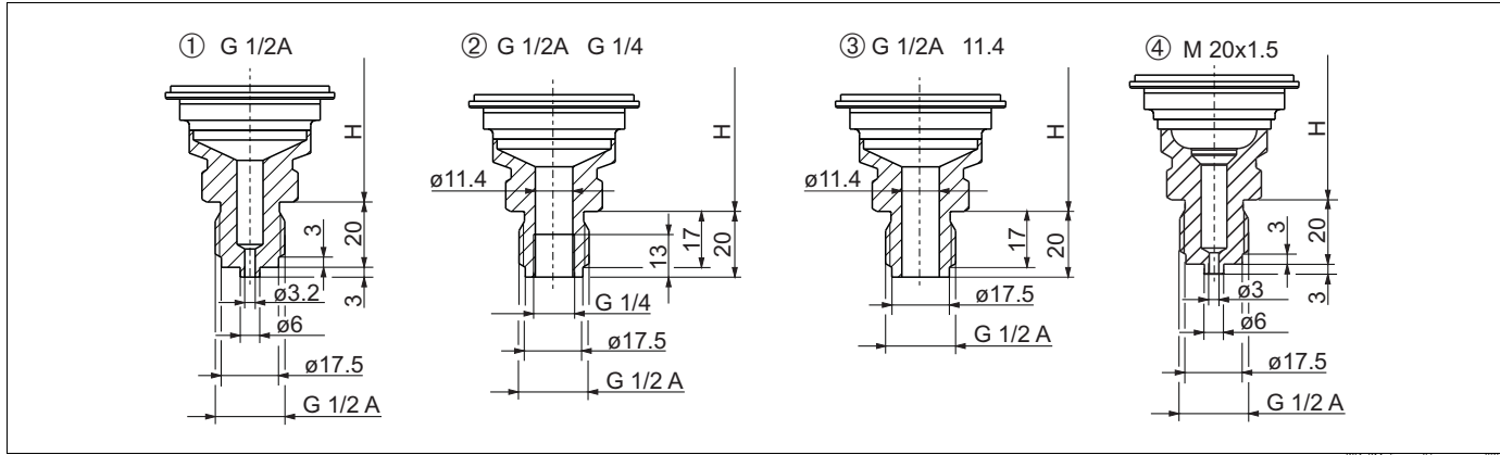
Process connections PMP51, thread ISO and DIN Installation height H \rightarrow 42.
