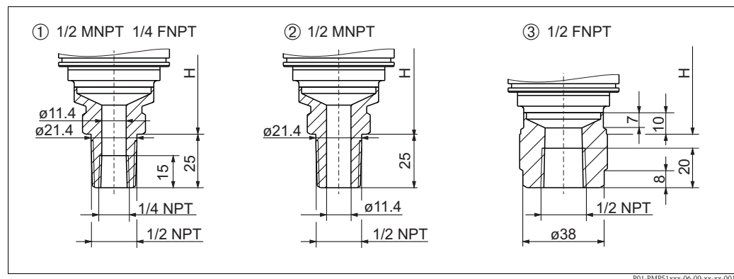
Process connections PMP51, thread ANSI Installation height H \rightarrow 42.
