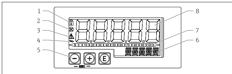
11 Display and operating elements of the process display unit
