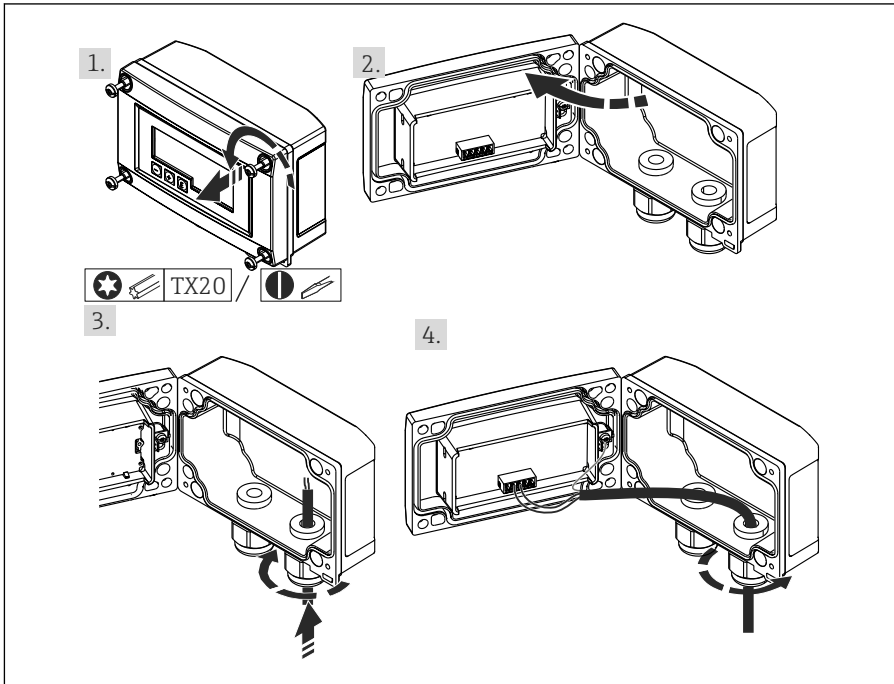
7 Inserting the cable, field housing
