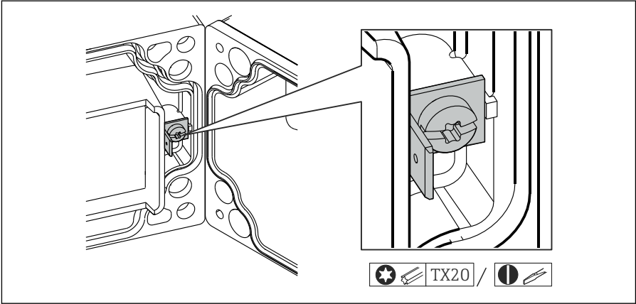
9 Functional grounding terminal in field housing
